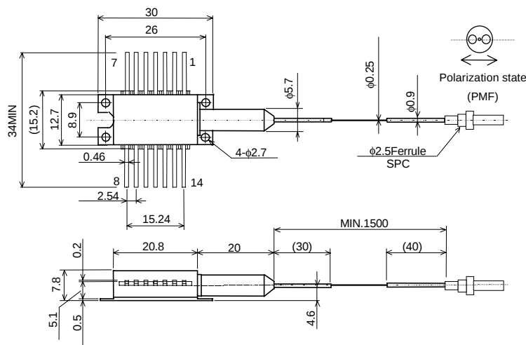
Package outline(Unit:mm) Type:AF4A1142A75L
